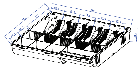
Unequal-5-Bill Tray
