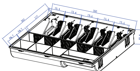
Equal-5-Bill Tray
